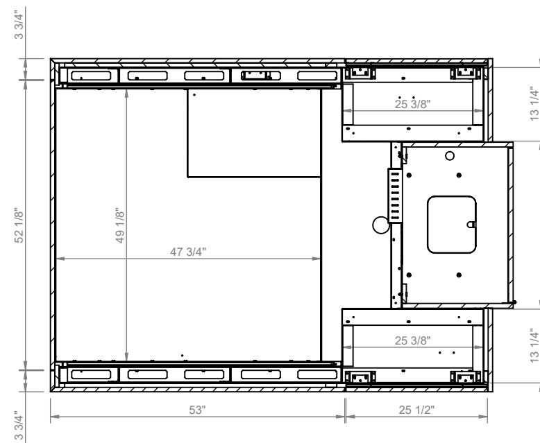
LOWER STORAGE VIEW SECTION B-B SCALE 1:24
