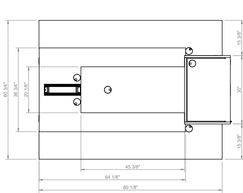
OVERVIEW SECTION A-A SCALE 1:24
